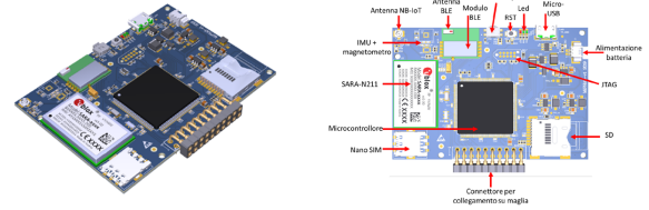
Figure 4: The preliminary prototype of MiPHAS hardware component
