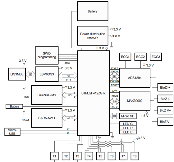
Figure 3: General architecture of the MiPHAS hardware component.
