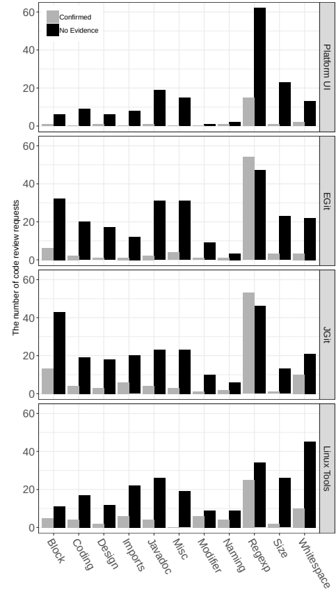
Fig. 5. The numbers of code review requests in which violations were addressed during code review (‘Confirmed’ – grey) and violations disappeared without evidence (‘No Evidence’ – black)
