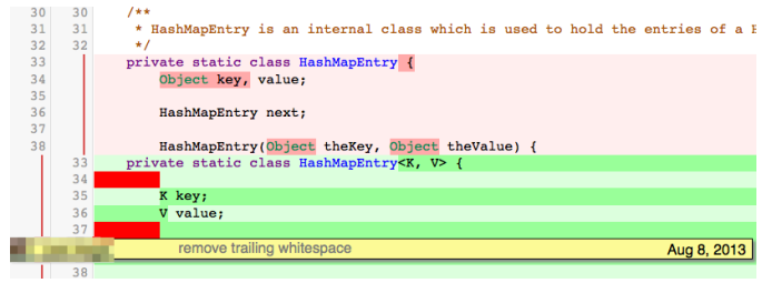
Fig. 7. A reviewer pointed out trailing whitespace during code review. Gerrit highlights trailing whitespace in red.
